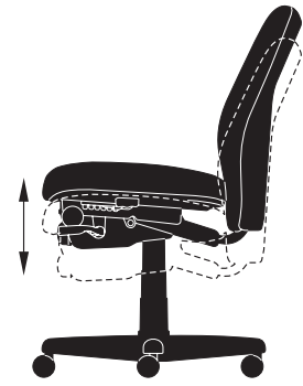
Pneumatic Seat Height Adjustment 4 3 / 4 " Range (16" - 20 3 / 4 ")
