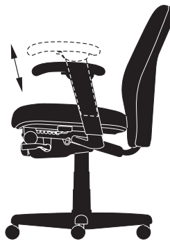
Adjustable Height Arms 4" Range (6" - 10" above seat)
